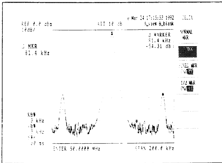
Figure 5.3-2 Delta Marker
