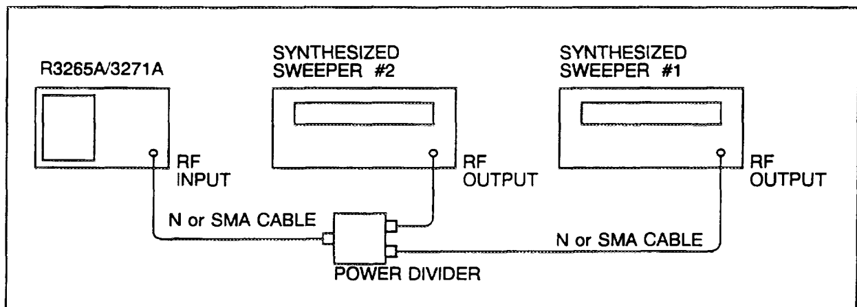
Figure 4-12 Third Order Intermodulation (<300 MHz) Test Setup
