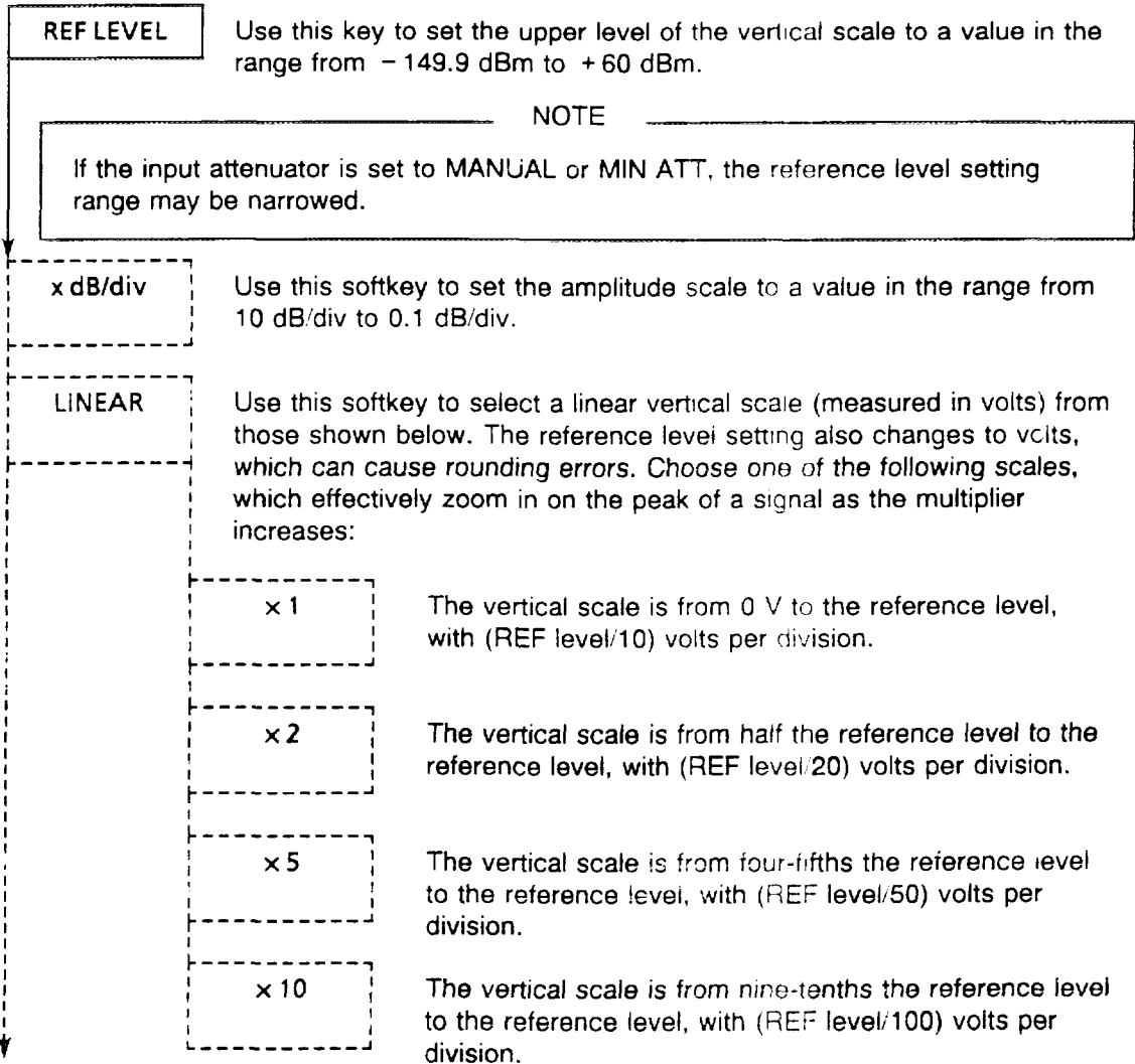
Figure 5.1-5 Reference Level
