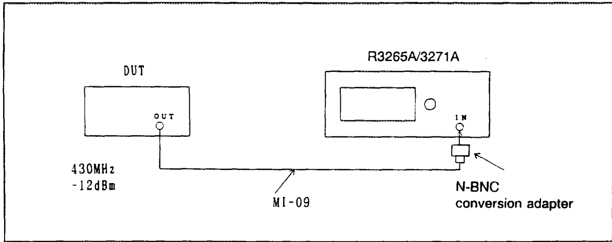
Figure 3-2 Wiring
